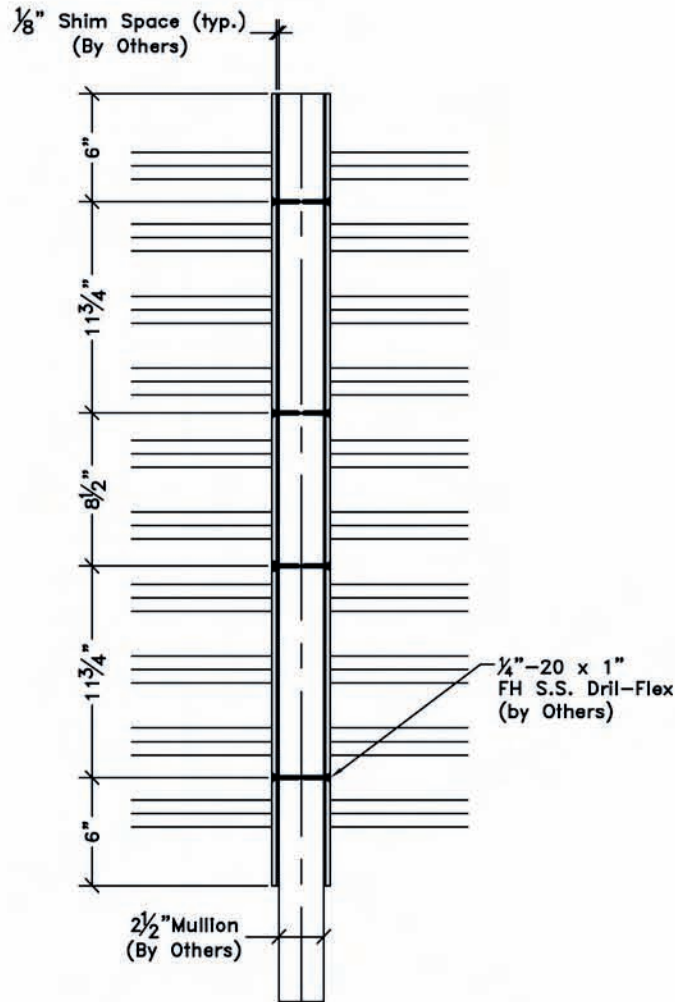
2a Typical Connection Detail Elevation View
