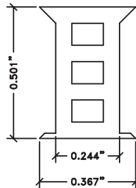
E-Z GLAZE SOUND STRIP 1/4" GAP FOR 1/2" THICK GLASS
