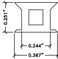
E-Z GLAZE SOUND STRIP 1/4" GAP FOR 1/4" THICK GLASS
