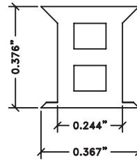
E-Z GLAZE SOUND STRIP 1/4" GAP FOR 3/8" THICK GLASS
